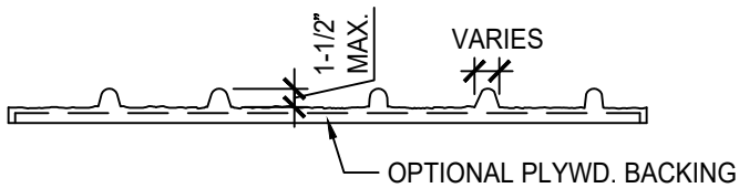
FORM LINER SECTION VIEW: A
