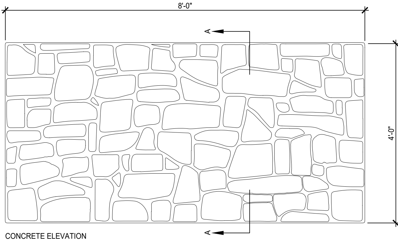
CONCRETE ELEVATION
