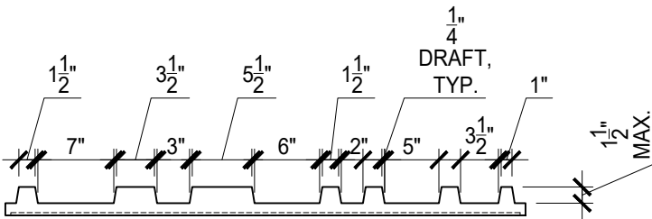
FORM LINER SECTION VIEW: A
