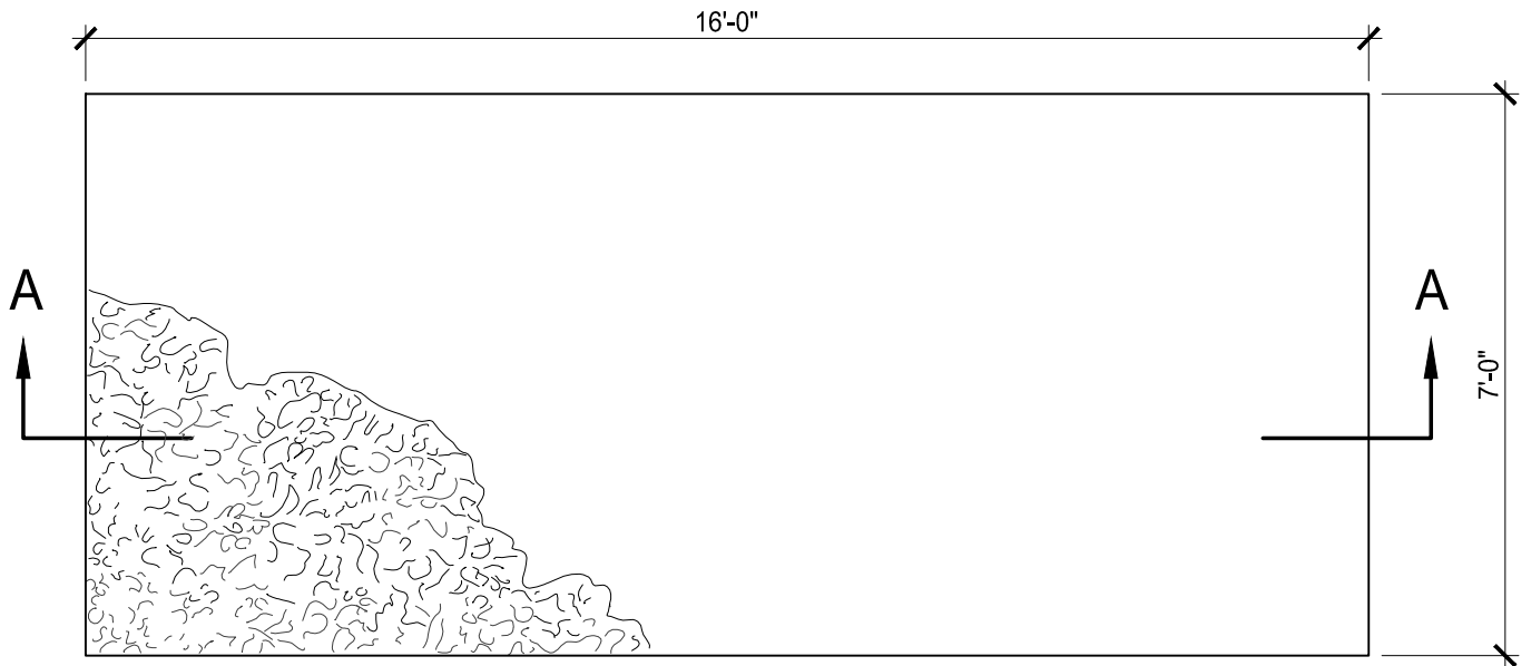
CONCRETE ELEVATION: F4T
