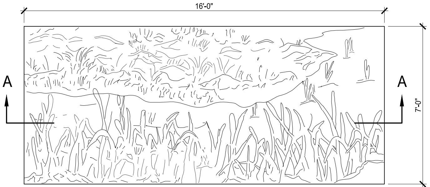
CONCRETE ELEVATION: F4B
