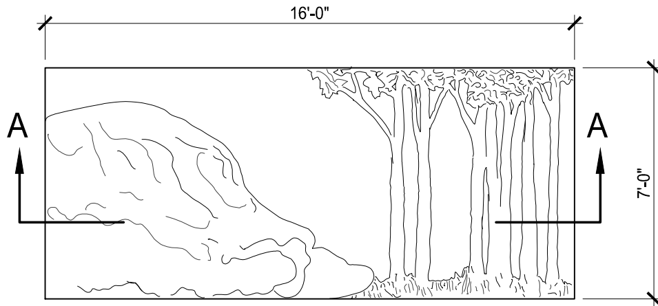
CONCRETE ELEVATION: S4BM-B
