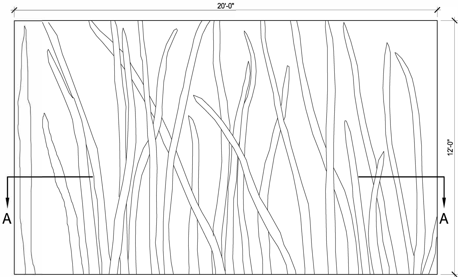
CONCRETE ELEVATION
