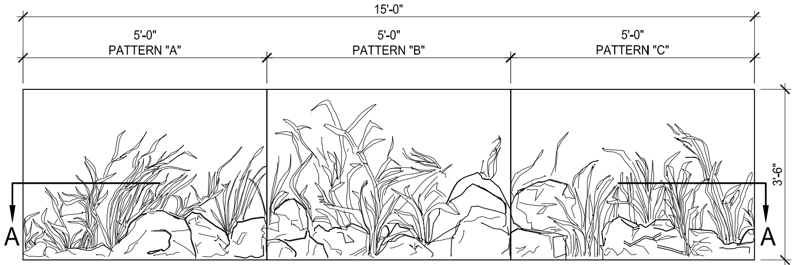
CONCRETE ELEVATION
