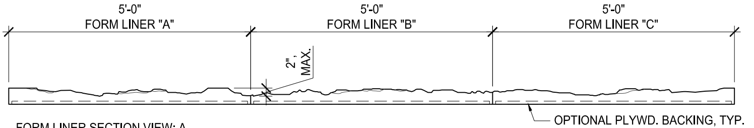
FORM LINER SECTION VIEW: A
