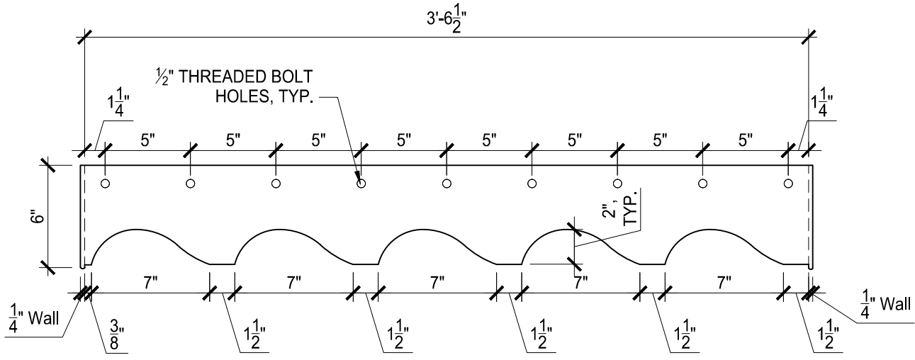
ELEVATION: SIDE A
