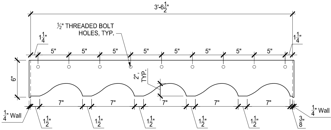
ELEVATION: SIDE B
