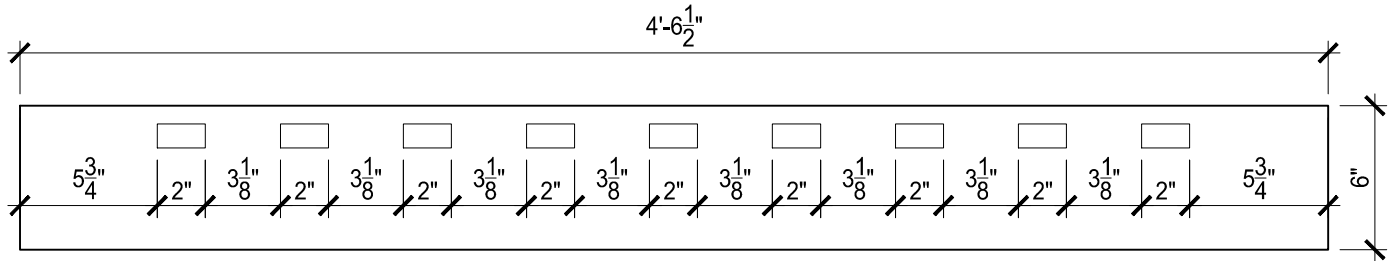
ELEVATION SIDE C:
