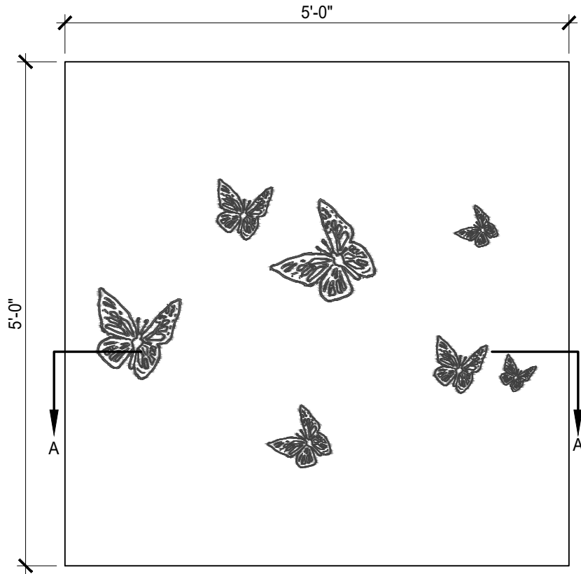
CONCRETE ELEVATION
