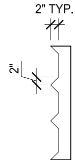
FORM LINER SECTION VIEW: A
