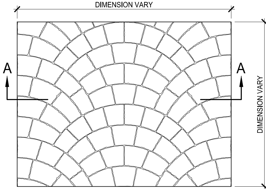
CONCRETE ELEVATION
