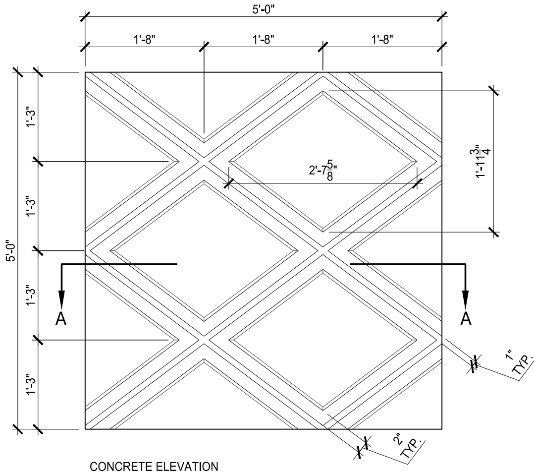
CONCRETE ELEVATION
