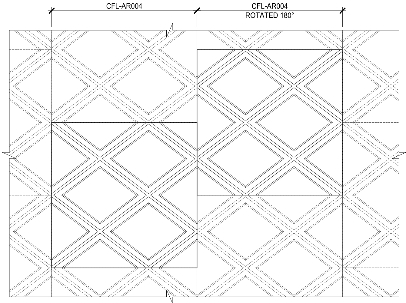
SAMPLE LAYOUT: MSE WALL
