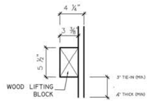
SECTION - B
