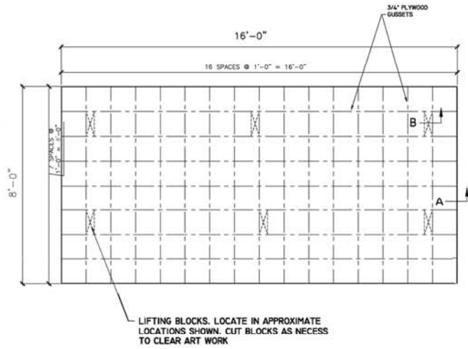
PLAN VIEW BACK
