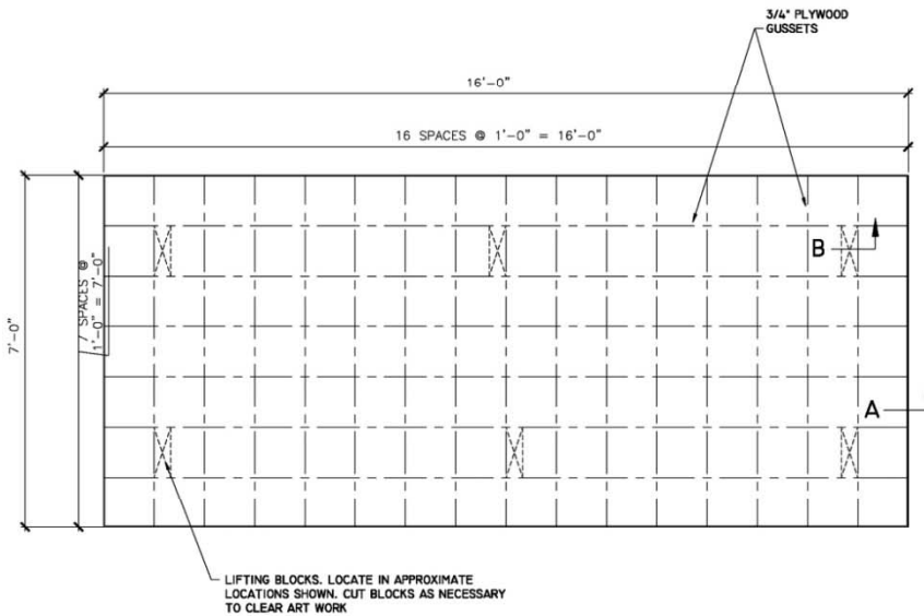
PLAN VIEW BACK
